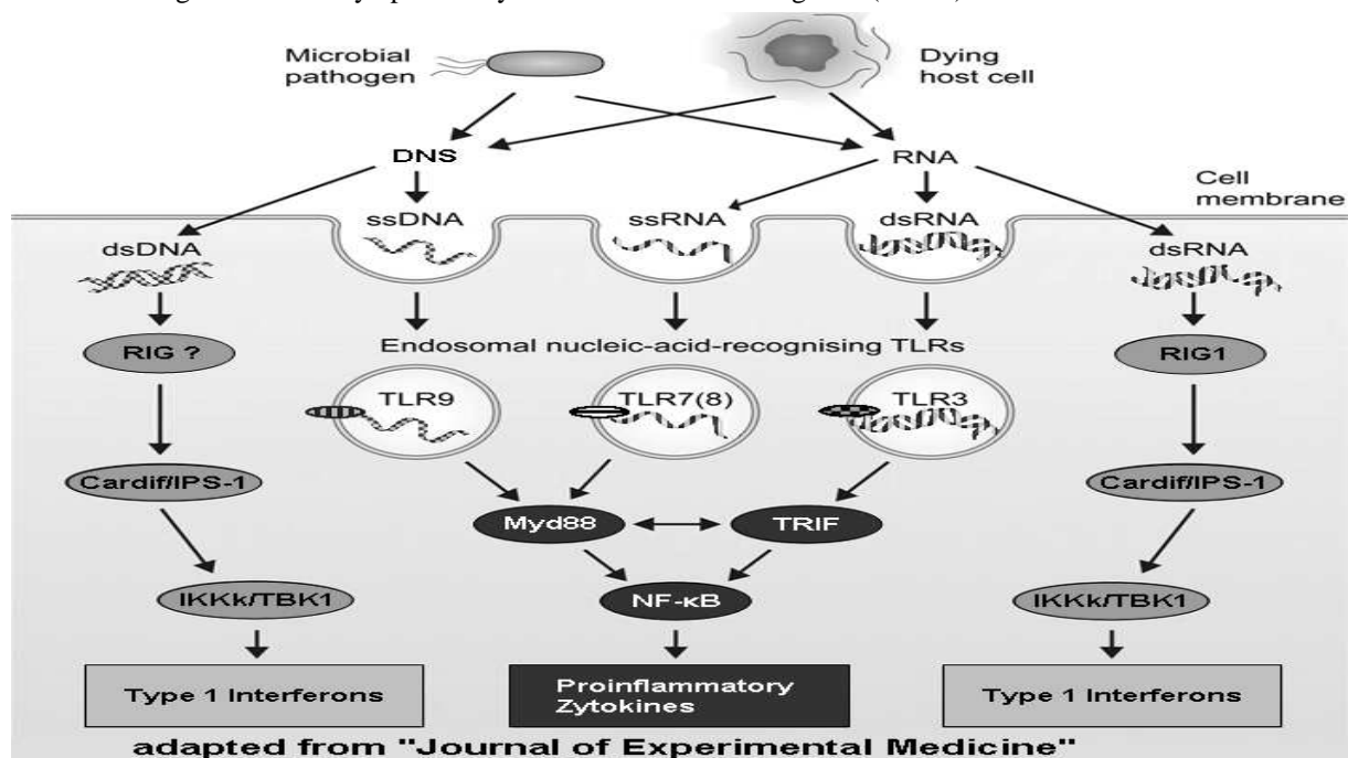
Figure 2: DNA/RNA recognition pathways in innate immune cells (WAGNER and BAUER (2006))
